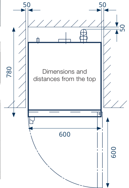
External dimensions of the station (W x D x H): 600 x 780 x 1945 / 2030 mm (varies due to adjustable feet)
